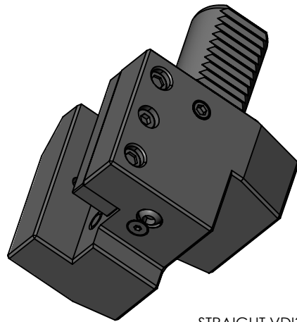
STRAIGHT VDI30 STATIC TOOL OUTPUT: 3/4" SQR SHANK COOLANT: EXTERNAL
